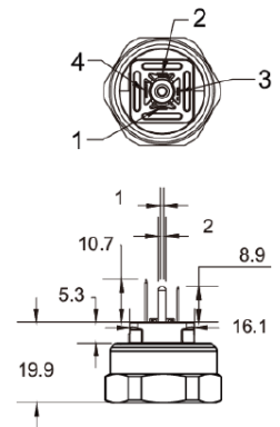
DC - EN17530-803 Form C (DIN 43650 Form C)
