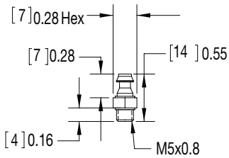
4mm 宝塔型接头 (x 2) (适用于 4mm (0.156") I.D. 管路)
